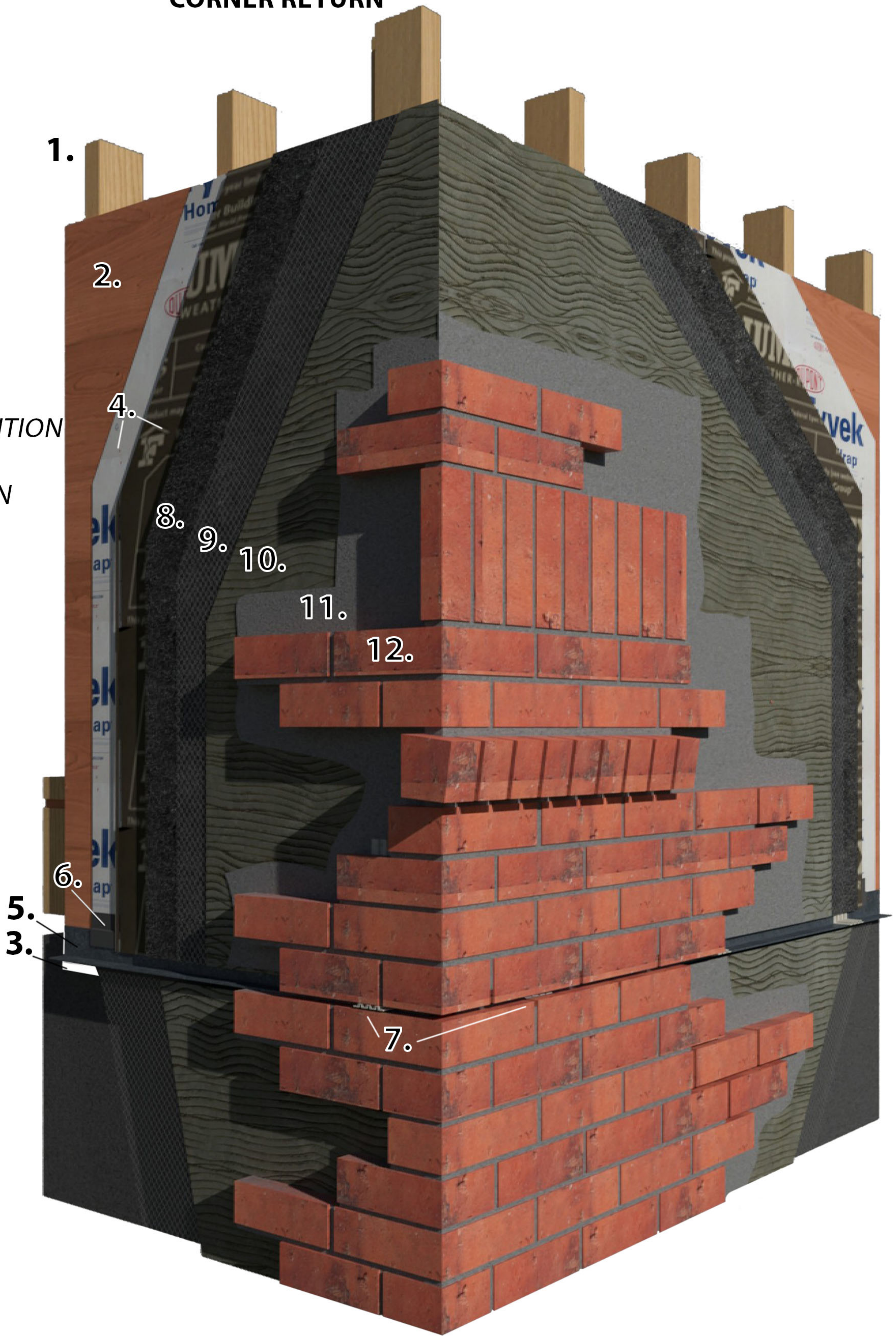
FIG. 3: THIN BRICK OVER WOOD FRAMING CONTINUING DOWN OVER FOUNDATION CORNER RETURN
